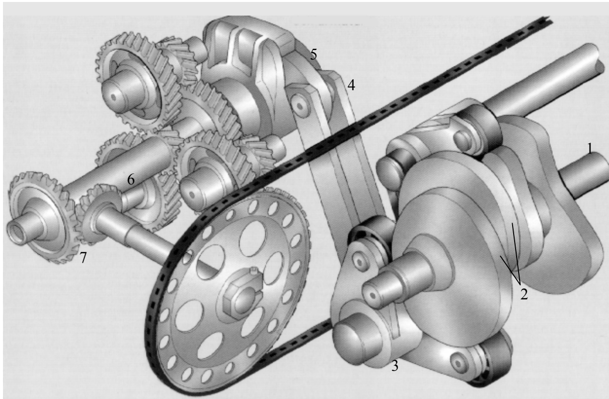
Fig. 40 – Driving system by double conjugated cams
