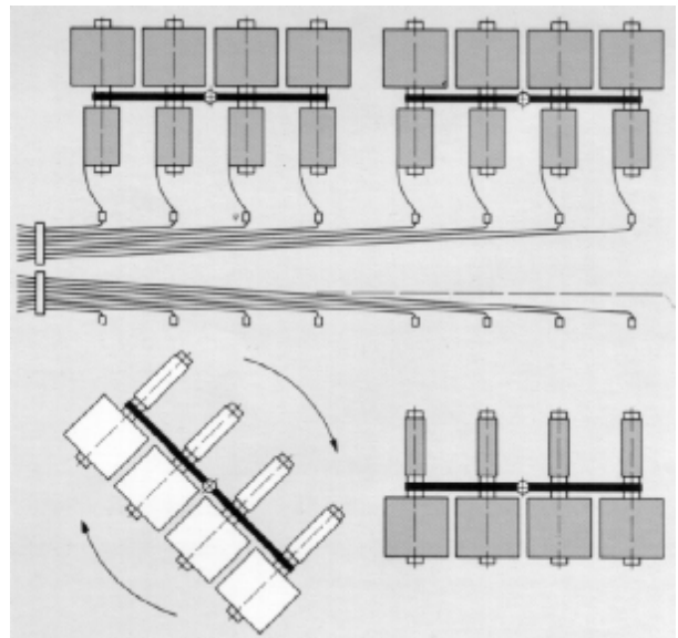
Fig. 3 – Swivel frame creel : this type of creel was designed as a variation of the mobile creel to enable the creeling up of bobbins which, owing to their heavy weight (5 to 25 kg), cannot be pinned on trolleys. Each bobbin holder is double-sided: the threads are unwound from one side, while a new series of bobbins is creeled up on the other side.
