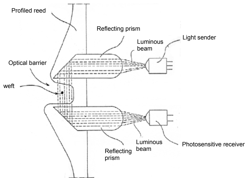
Fig. 109 – Optical sensor applied on an air jet weaving machine
