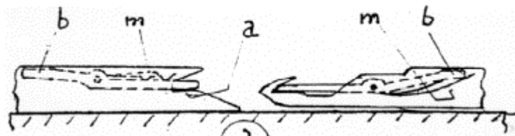
Fig. 37 – Negative rapier exchange
