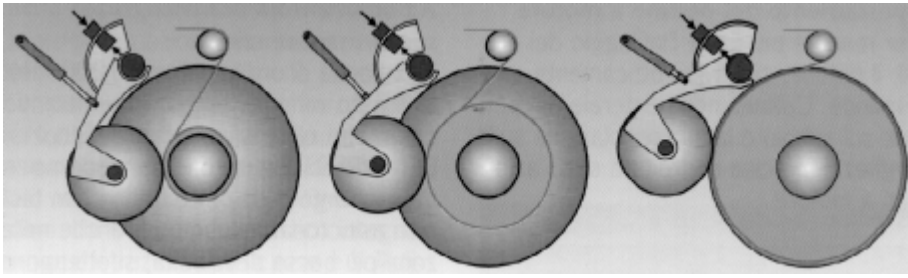
Fig. 20 – The increasing winding thickness of the yarn on the beam moves the pressure roller backwards.
