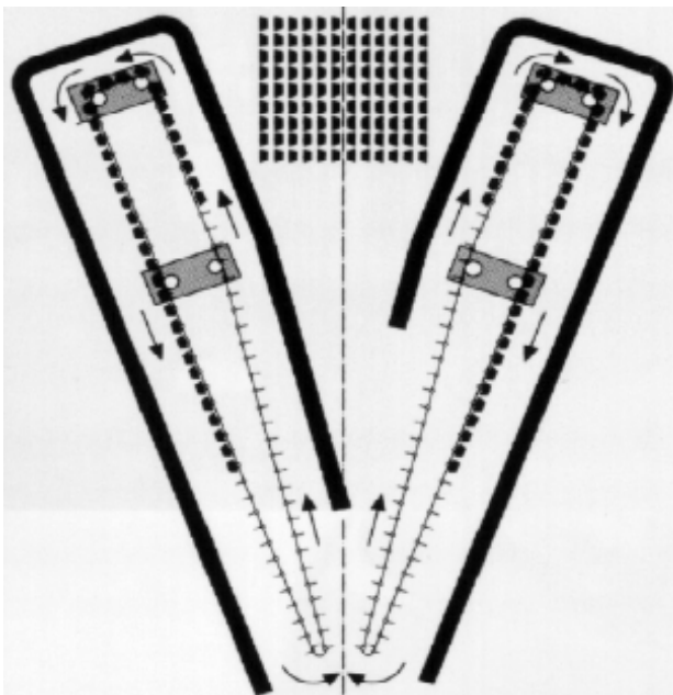
Fig. 3 – Swivel frame creel : this type of creel was designed as a variation of the mobile creel to enable the creeling up of bobbins which, owing to their heavy weight (5 to 25 kg), cannot be pinned on trolleys. Each bobbin holder is double-sided: the threads are unwound from one side, while a new series of bobbins is creeled up on the other side.
