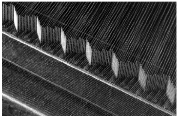
Fig. 19 – Expanding comb.
