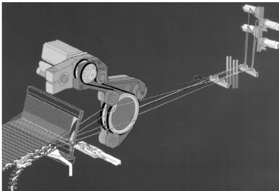
Fig. 116 – Double disk device for leno selvedges
