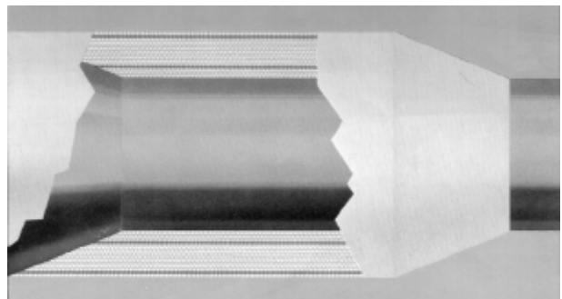
Fig. 11b – Correct winding up of the warp on the drum. Warping with same number of revolutions produces identical thickness of thread layers.
