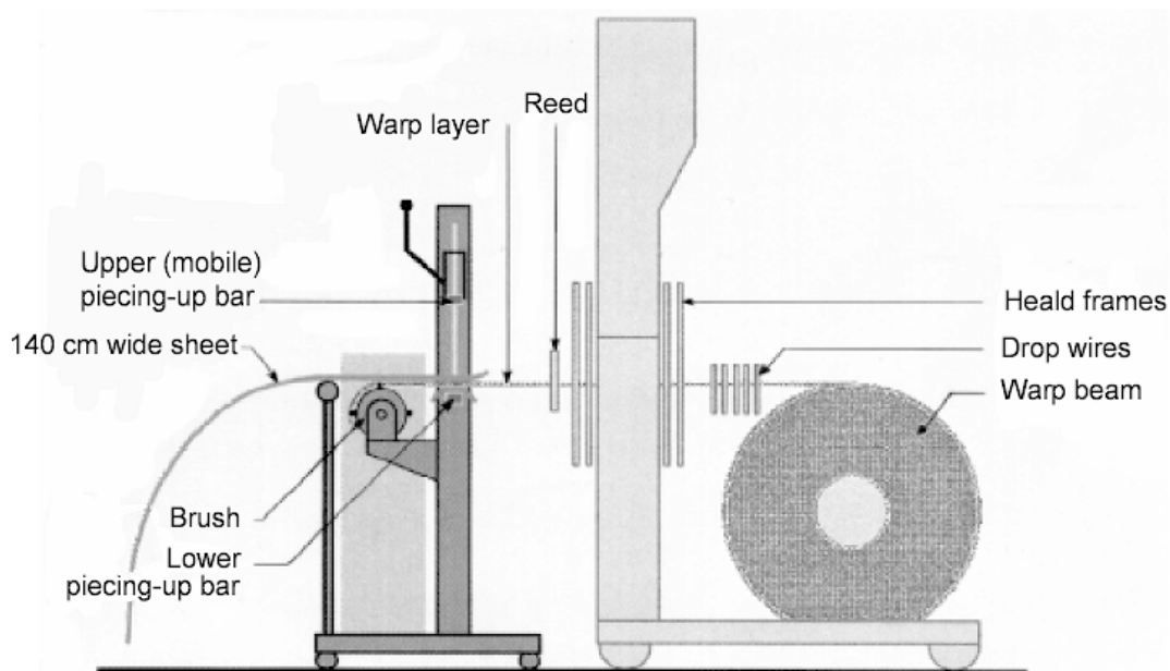
Fig. 32 – Piecing-up
