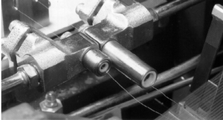
Fig. 61 – Insertion nozzles for 2 different threads
