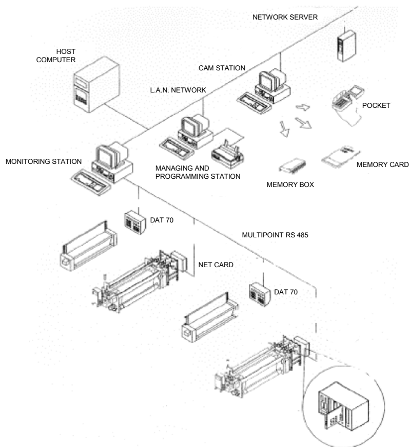
Fig. 92 – Example of a modern monitoring and control network
