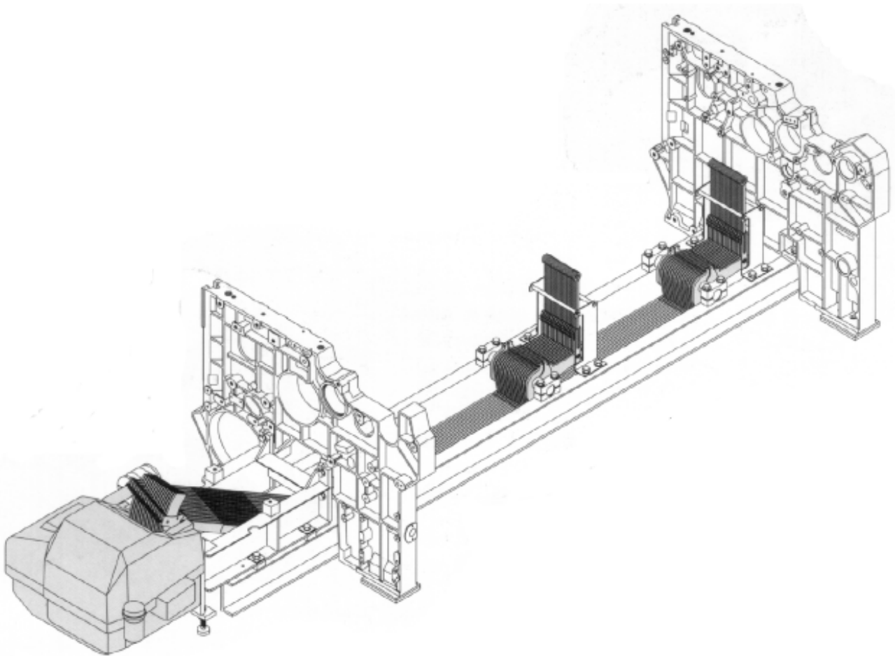
Fig. 74 – Skeleton of a weaving machine
