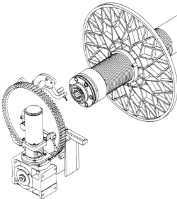
Fig. 98 – Quick beam change: this operation is facilitated by the quick insertion of the beam's end through grooved profile driven by an eccentric, while leaving the gear on board the weaving machine; the beam blocking is guaranteed by a quick gripping system
