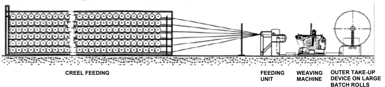
Fig. 101 – Weaving machine equipped with creel feeding and outer take-up device on large batch rolls (2000 mm diameter), used only for particular needs, like technical fabrics
