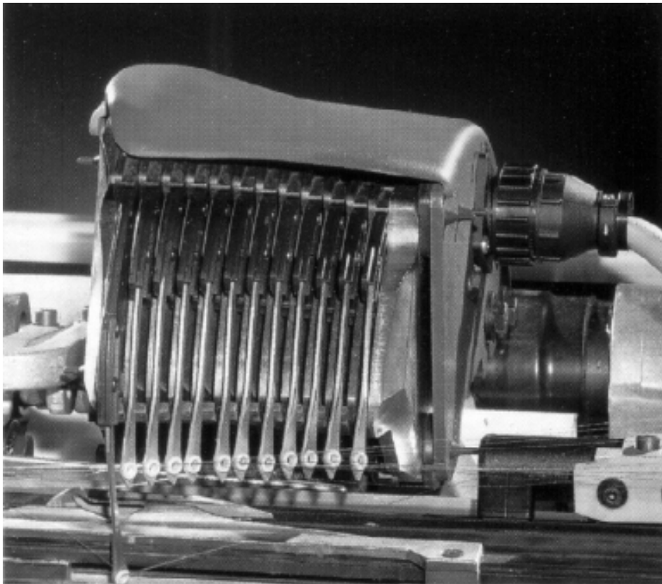
Fig. 44 – Colour selector with 12 bolts
