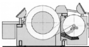
Fig. 16b – Beaming of staple yarns warps with pressure roll device.
