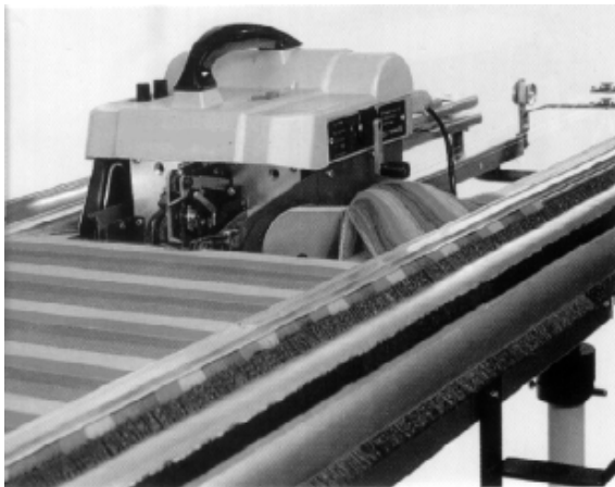
Fig. 33 – A knotting machine in operation on a warp with colour sequence, tensioned on the proper frame.
