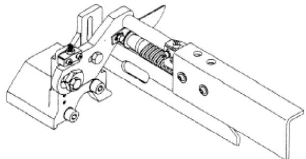
Fig. 99 – Quick temple positioning: this operation permits the immediate re-positioning of the temple during re-assembling
