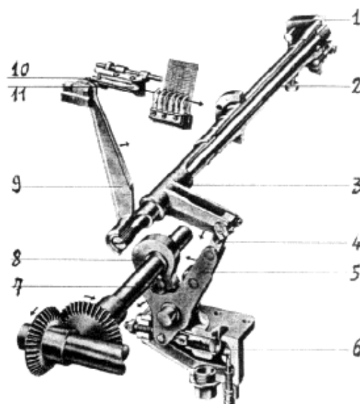
Fig. 48 - Projectile launching mechanism
