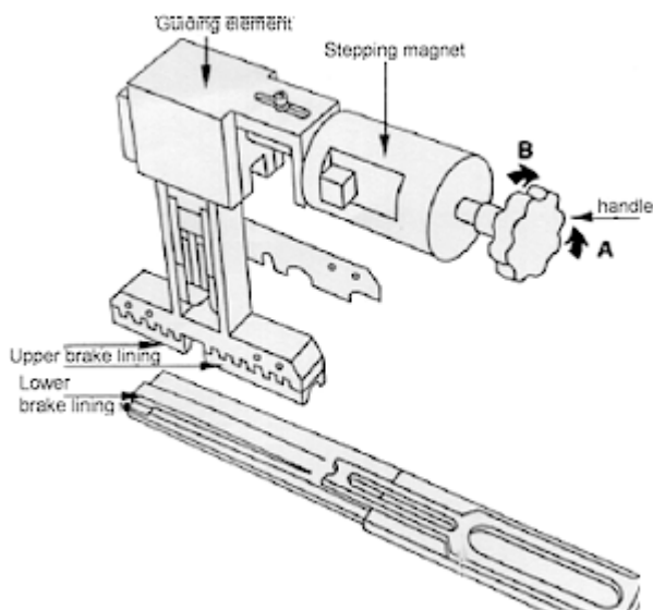
Fig. 51 – Projectile brake
