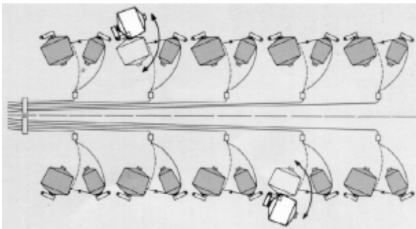
Fig. 2 – Magazine creel : this kind of creel is used when several warps of similar type must be prepared in sequence, that is when large lots of similar yarns need to be processed. Level with each tensioner, two bobbins are positioned: one operating and the other as reserve.
