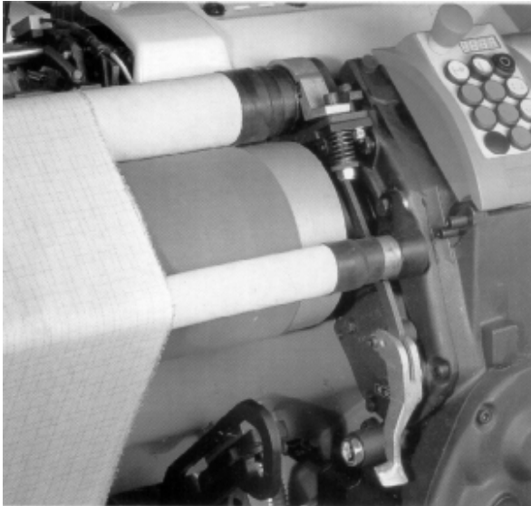
Fig. 79 – Take-up motion and guide/pressure rollers for the fabric take-down, which has to take place without any slippage. For this purpose the surface of the take-up roller is covered with an emery cloth and, when weaving delicate fabrics, with rough or smooth rubber
