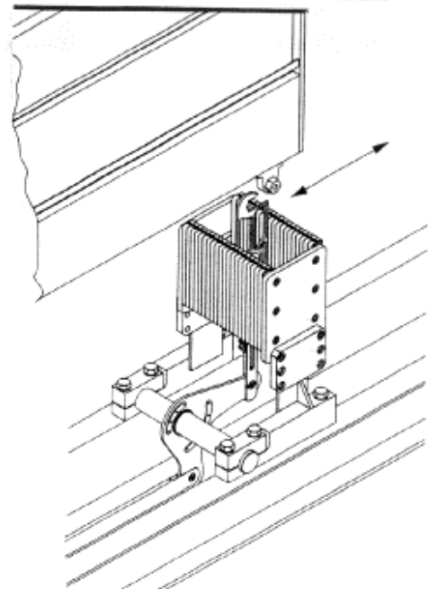
Fig. 97 – Quick heald frame hooking: this operation permits quick hooking and unhooking of the heald frames by their lateral shifting, avoiding manual operations in the zone below
