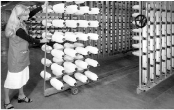
Fig. 1 – Mobile creel : this creel type is similar to the standard creel, but is formed by trolleys which can be taken individually out of the creel. The bobbins are creeled up on each trolley outside the creel. During the creeling up of a series of trolleys, the second series of trolleys is brought back to the outside of the creel to feed the warper. This reduces considerably the waiting time. The mobile creel comes in handy especially when there is insufficient room to permit the use of two standard creels.
