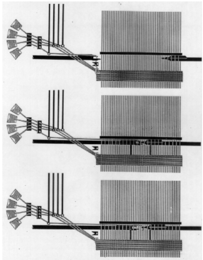
Fig. 36 – Working principle of a rapier weaving machine.
