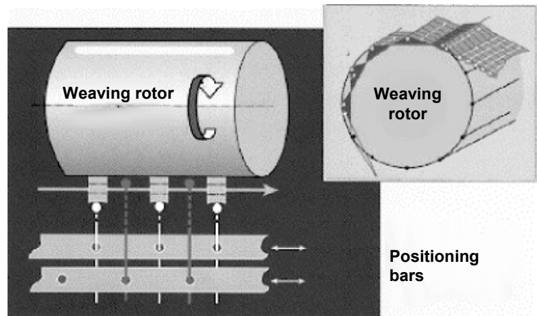
Fig. 104 – The elements of the weaving rotor form, by plunging one after the other into the warp yarn sheet, forming a sequence of sheds. The positioning bars select the threads to be raised through movements of only few millimetres.
