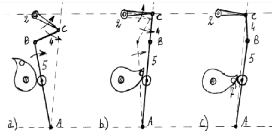
Fig. 49 – Loading of the torsion bar: a) torsion bar 2 in rest, knee-joint lever 4+5 in articulate position; b) loading phase; c) torsion bar in tension and knee-joint lever in stable position, before the launching control by roller 7.
