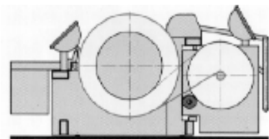
Fig. 16a – Beaming of continuous filament warps without pressure roll device.
