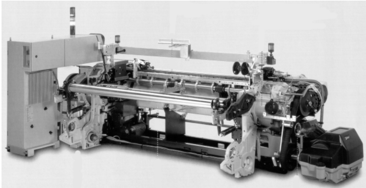
Fig. 75 – Skeleton of a weaving machine with various already mounted components
