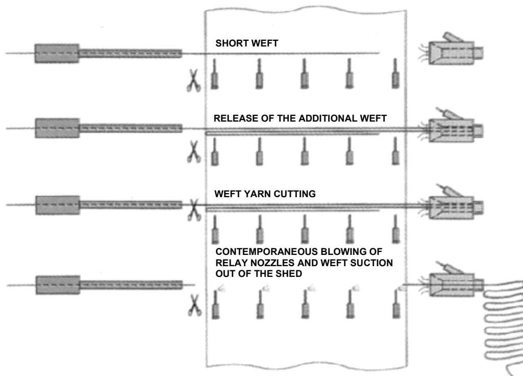
Fig. 59 – Automatic weft repair
