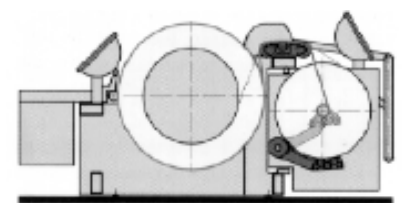
Fig. 16c – Beaming of staple yarns warps with waxing device, with or without pressure roll device.
