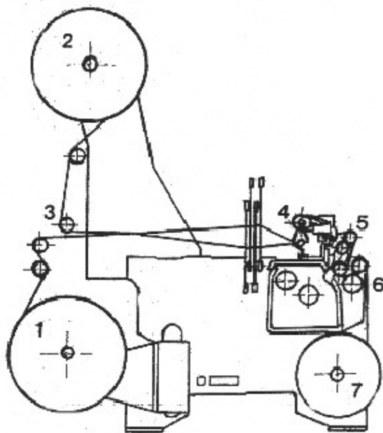
Fig. 64 – Terry weaving machine:
