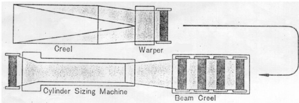
Fig. 26 – Conventional sizing: Creel: contains the cones Warper: warps the threads Beam creel: contains the beams Cylinder sizing machine: sizes the yarn
