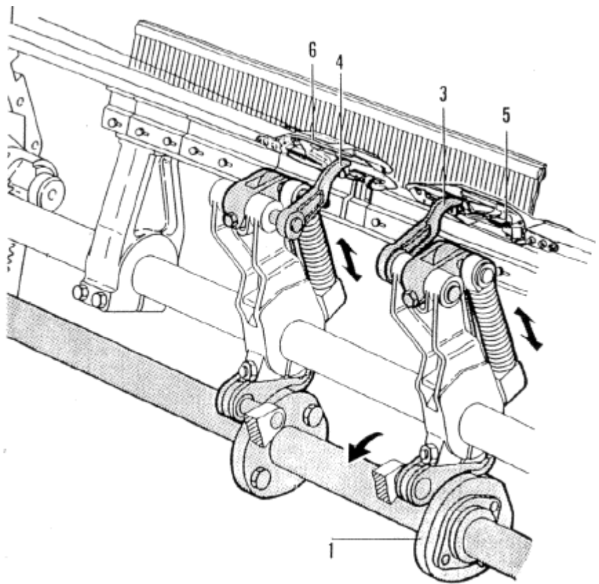
Fig. 38 – Positive rapier exchange
