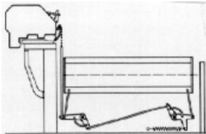
Fig. 84 – Negative dobby (upper position for water-jet weaving machines)
