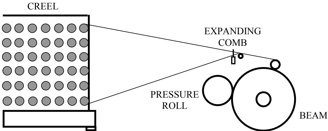
Fig. 18 – Beam warping machine.
