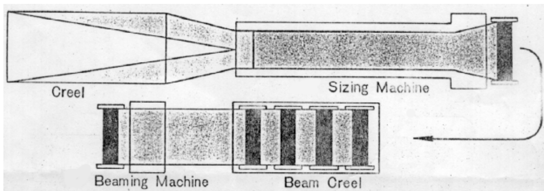
Fig. 27 – Unconventional sizing: Creel: contains the cones Sizing machine: warps and sizes the yarn Beam creel: contains the already sized beams Beaming machine: assembles the threads of the sized beams and forms the warper's beam.
