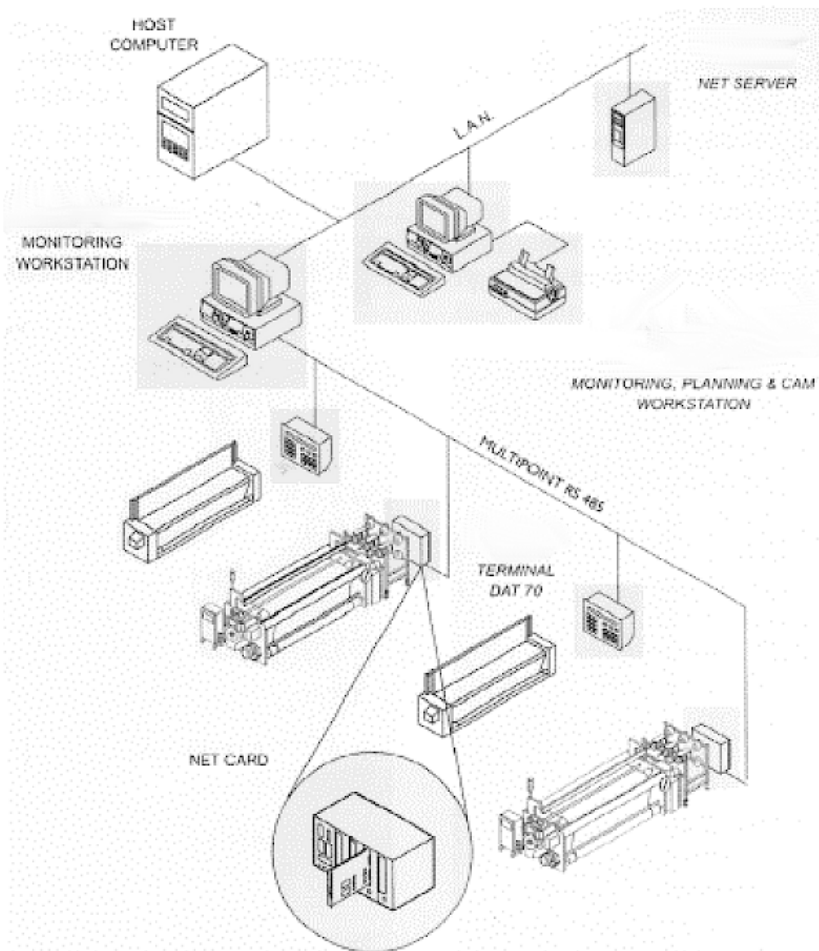
Fig. 118 – Advanced monitoring system
