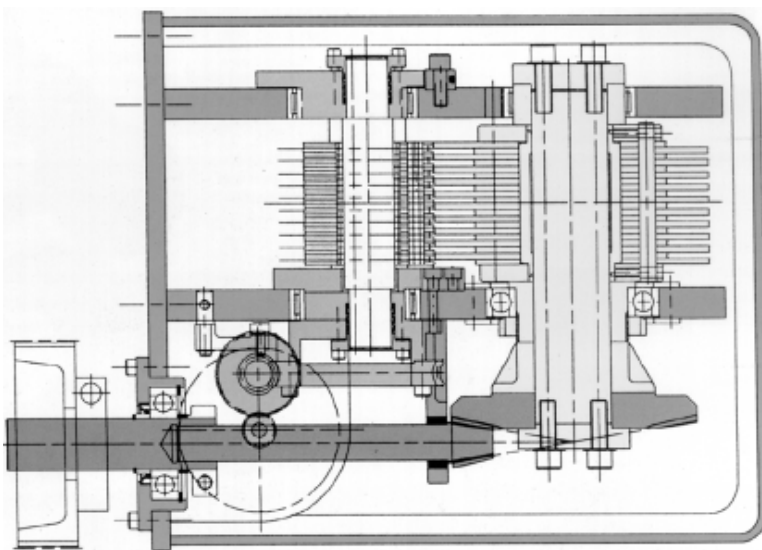
Fig. 82 – Conjugated cams with roller lever
