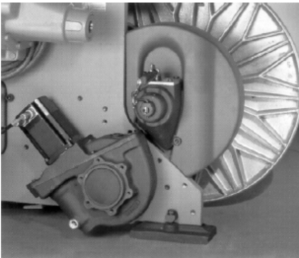
Fig. 77 – Servomotor for let-off motion drive
