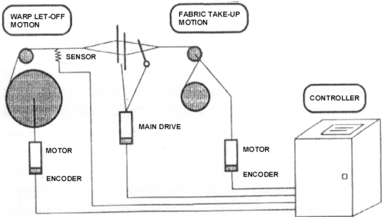
Fig. 76 – Integrated system with electronic control “operating in series” of the warp let-off and of the fabric take-up motions
