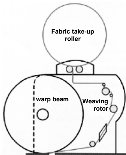
Fig. 103 – Structure of the multiphase multilinear weaving machine
