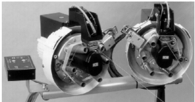
Fig. 107 – Pre-feeders for water jet machine with microprocessor controlled weft selection
