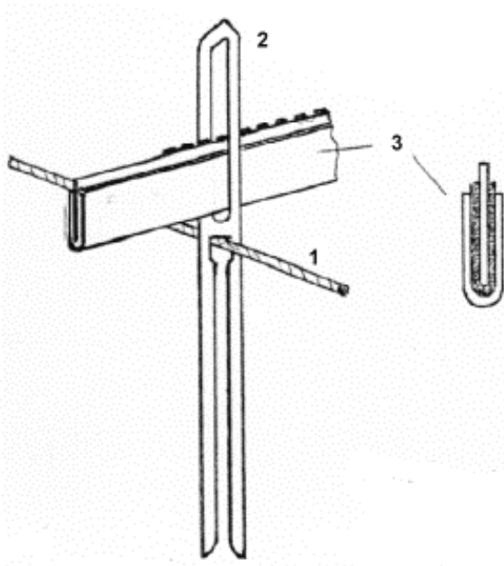
Fig. 110 – Electric warp stop motion:
