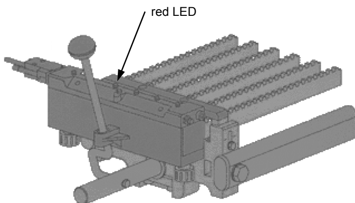
Fig. 113 – An electronic device signals by the lighting of a light-emitting diode placed at the end of each contact rail the bar and its half on which the drop wire has fallen.
