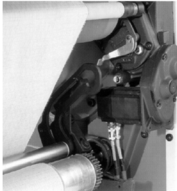
Fig. 78 – Servomotor for take-up motion drive
