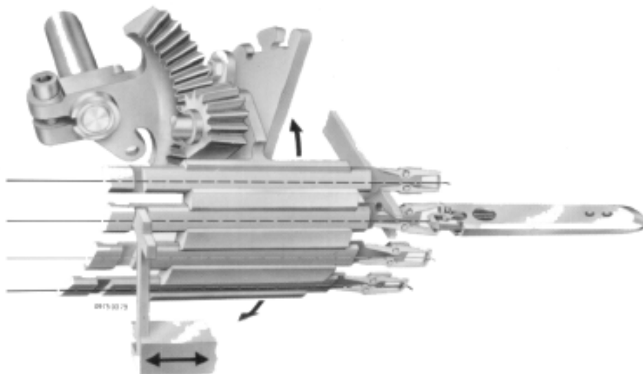
Fig. 53 – Colour selector
