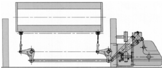
Fig. 81 – Assembly scheme of the cam machine
