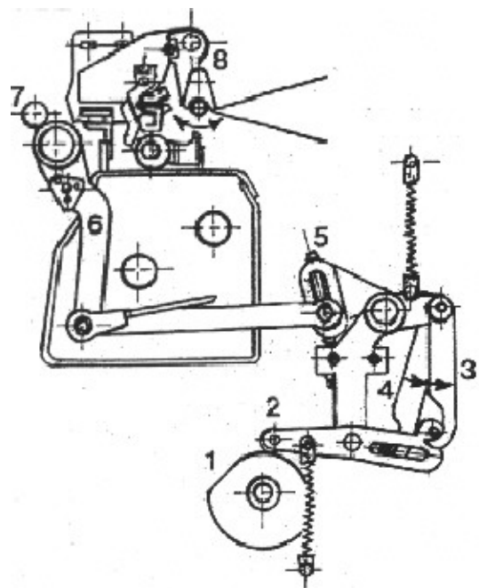
Fig. 65 – Terry weaving machine: fabric motion gear
