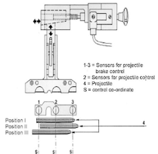
Fig. 52 – Brake adjustment
