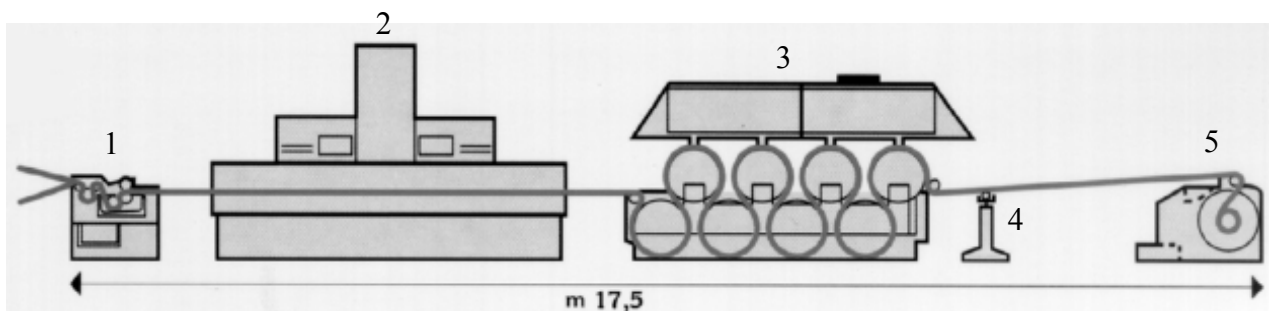
Fig. 24 – Sizing machine : 1 – Size vat; 2 – Radio-frequency oven; 3 – Drum drying machine; 4 – Waxing device; 5 – Beaming.
