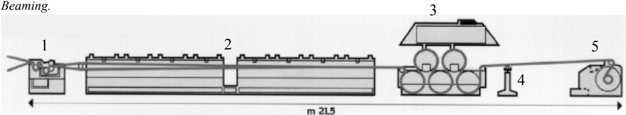
Fig. 25 – Sizing machine : 1 – Size vat; 2 – Hot air oven; 3 – Drum drying machine; 4 – Waxing device; 5 – Beaming.
