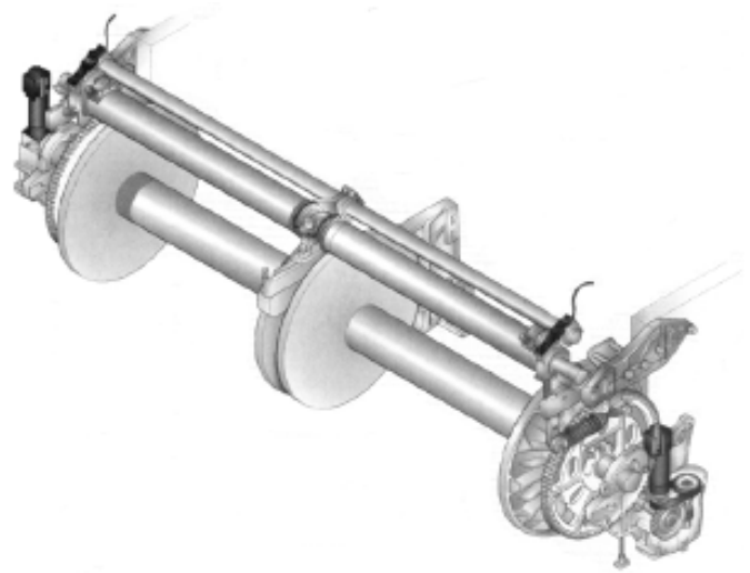
Fig. 80 – Example of double warp let-off motion for heavy weight fabrics or for fabrics with high warp yarn density (double width sizing machines and double capacity beam carriers would be required): the tension detecting system is independent on the two half-beams
