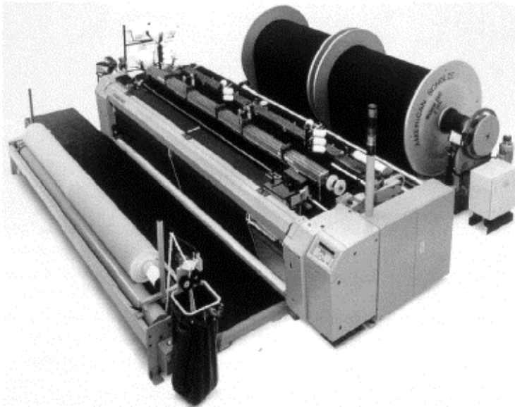
Fig. 100 – Projectile machine equipped with outer winding unit into large batch rolls and with double outer beam of large size (1600 mm). This ensures maximum warp duration, good accessibility and easy operation
