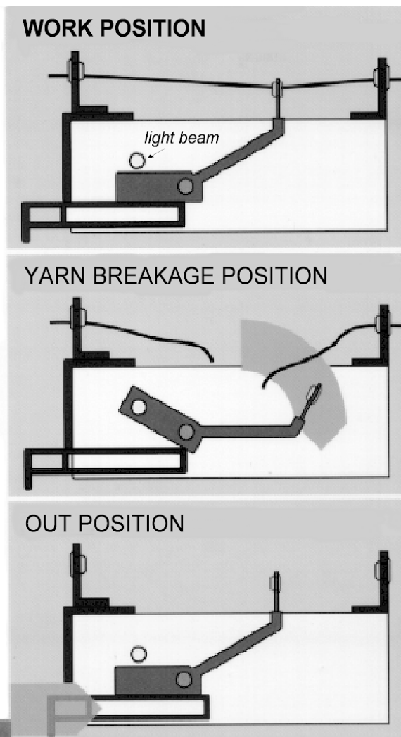
Fig. 5a – During warping the thread supports the drop pin and the light beam is not interrupted.
