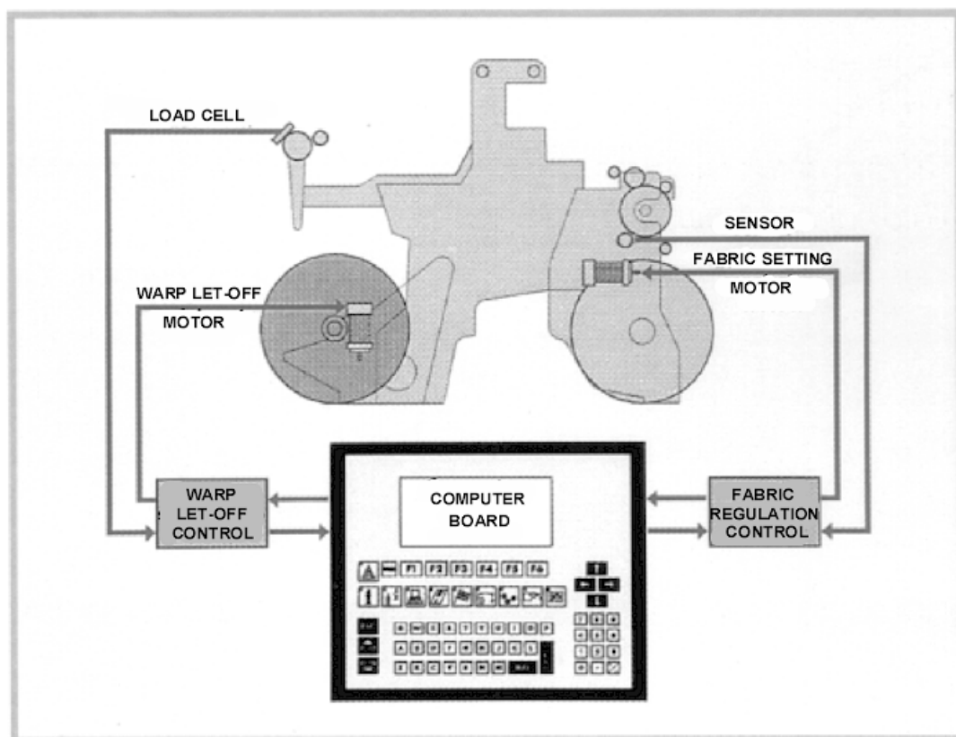
Fig. 93 – Electronic detecting and control system on thread tension. Setting and modification of tension and weft density directly via board computer
