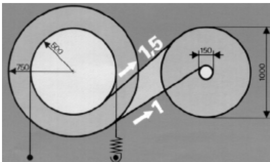
Fig. 14 – Variation of the diameter ratio during beaming. Without the automatic adjustment of the warp tension, this would increase by about 50%.
