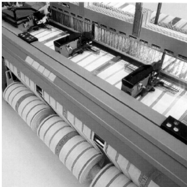
Fig. 117 – Devices for centre selvedge formation in a projectile weaving machine
