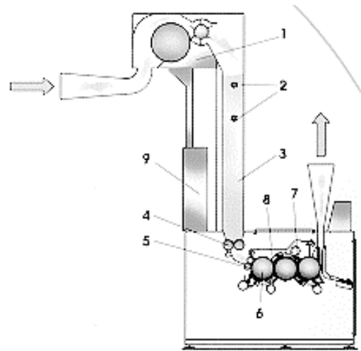
Fig. 12 Section view of three-cylinder opener
