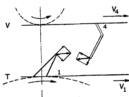
Fig. 140 Fibre raising
