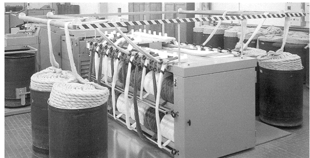
Fig. 198 – Feed rack
