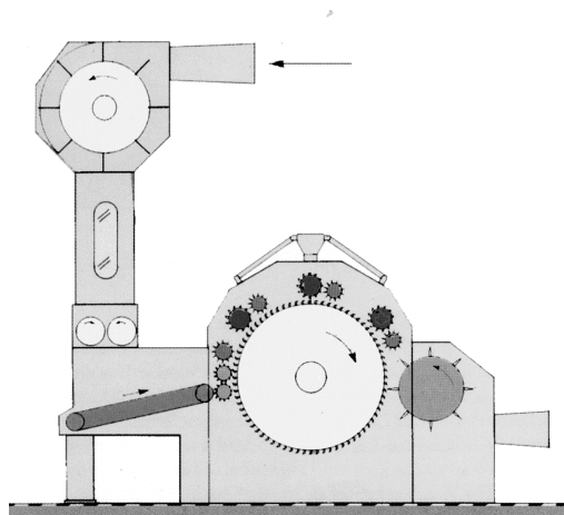
Fig. 72 Carding willow
