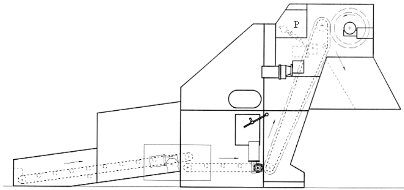
Fig. 108 - Automatic feeder
