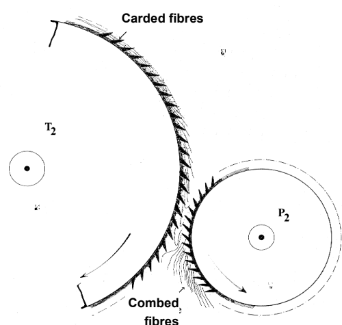
Fig. 153 – 2nd drum-comber roller
