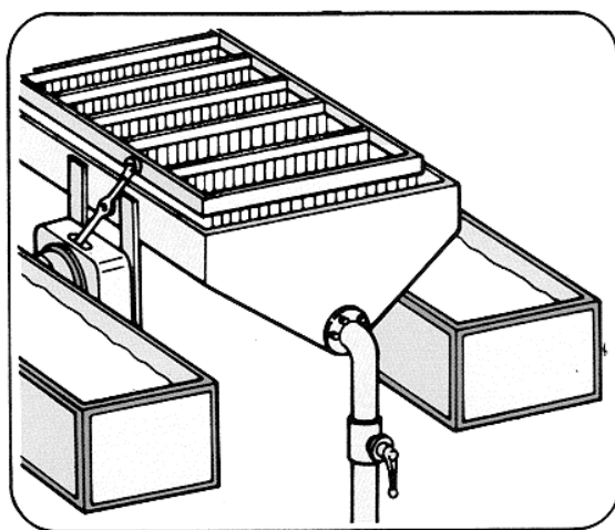
Fig. 119 – Scouring vats with two side settling troughs
