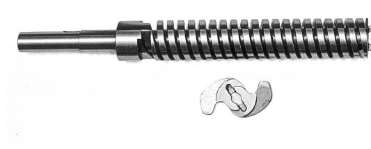
Fig. 170 - Screw and cams
