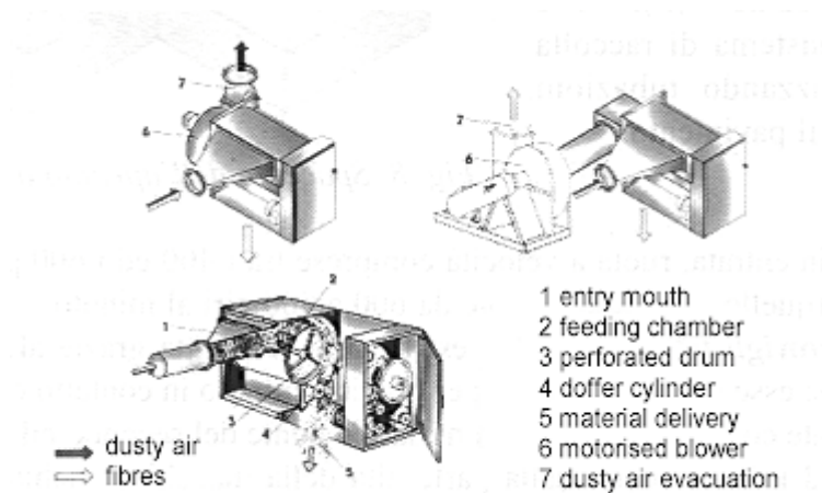
Fig. 7 Diagram and cut-away view of the aspiration cage
