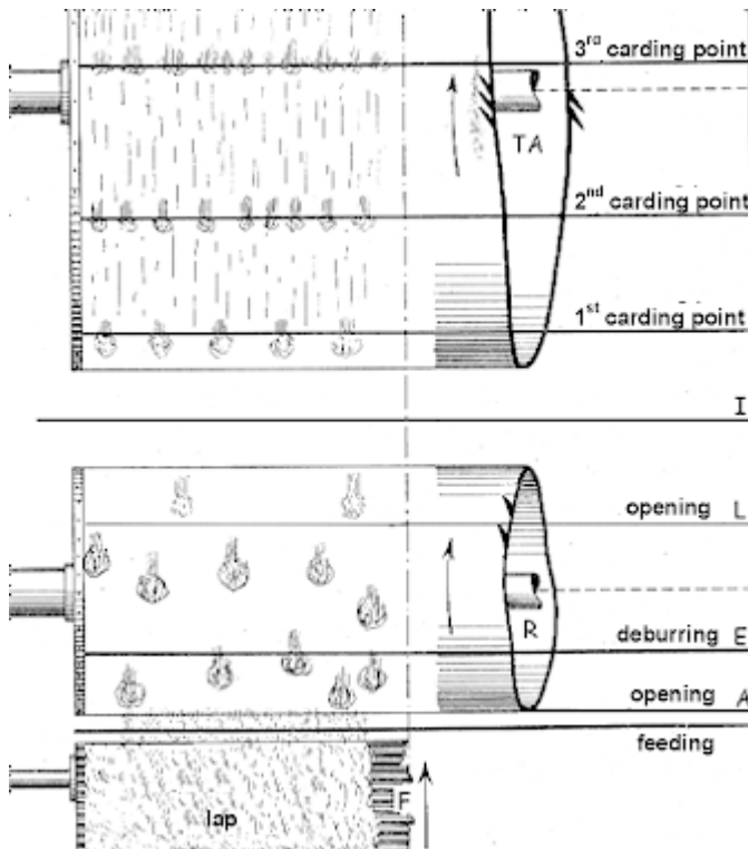
Fig. 144 – Feeding and opening the web
