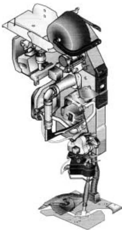
Fig. 57 Winding head
