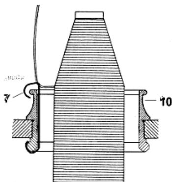
Fig. 214 – Ring and traveller
