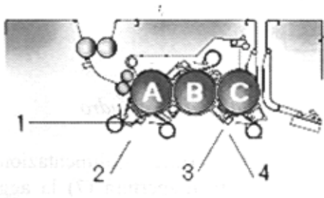
Fig. 13 Detail of the three-cylinder set
