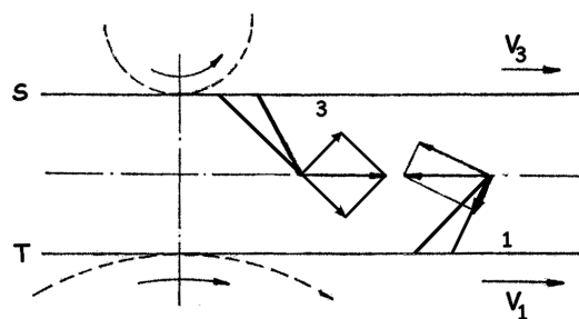
Fig. 137 Fibre transfer
