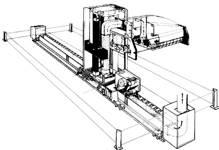
Fig. 5 A cut-away view of the bale plucker
