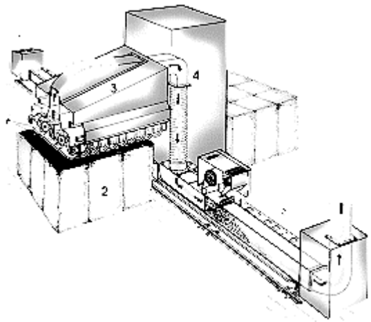
Fig. 2 Diagram of a bale plucker
