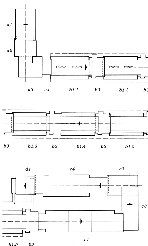
Fig. 106 – A complete scouring line
