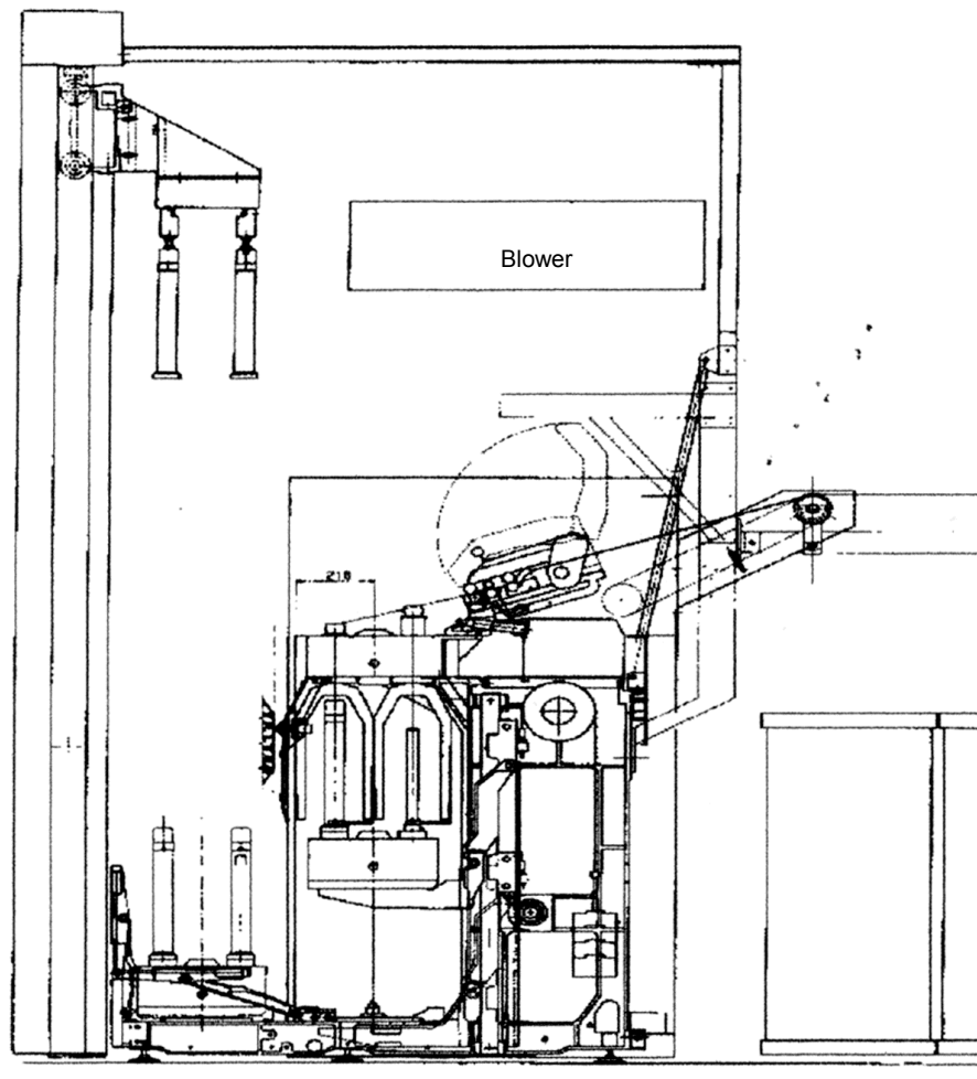
Fig. 44 Functional diagram of a roving frame
