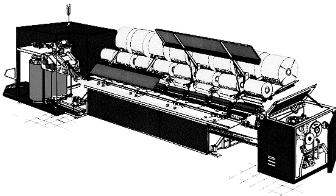
Fig. 31 Combing machine
