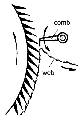
Fig. 139 Doffer comb
