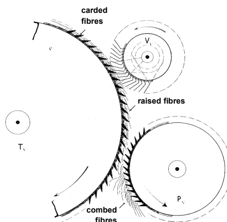
Fig. 156 The effect of the fly roller
