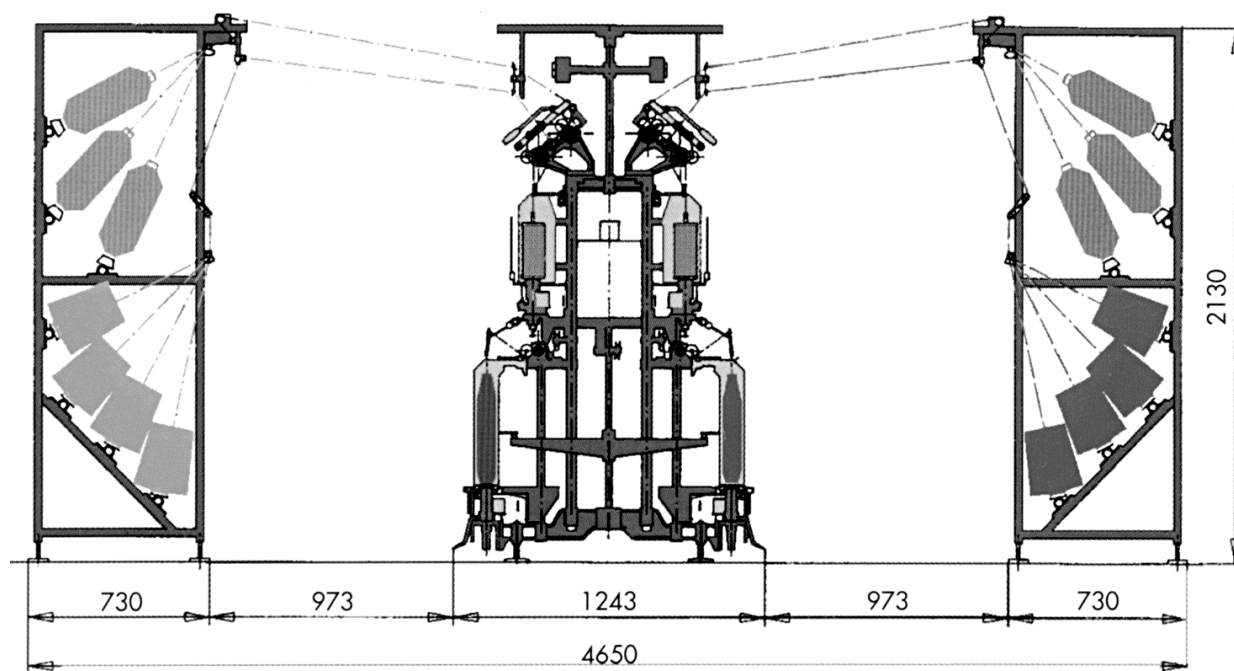
Fig. 103 Twisting machine
