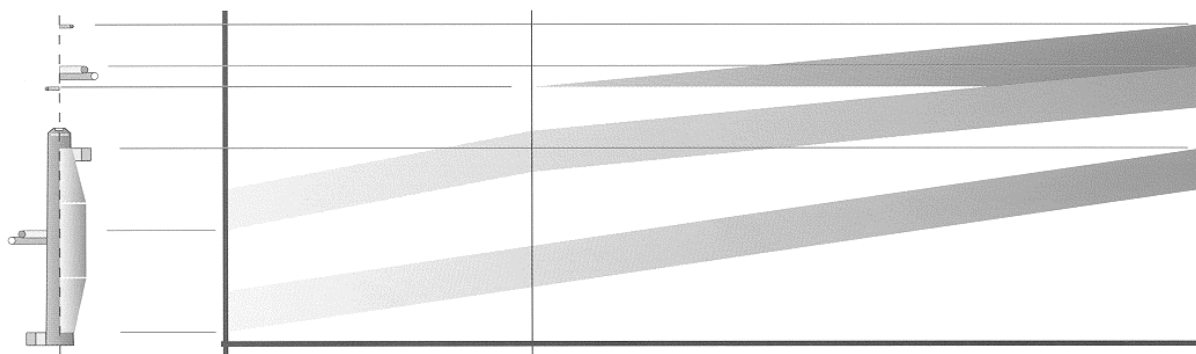
Fig. 222 – Synchronised motion diagrams of the ring rail, of the anti-balloon ring and of the yarn guide.
