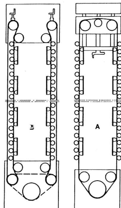
Fig. 218 – Tangential drive belt
