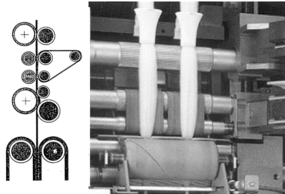
Fig. 208 – Control with barrel elastic-control rubber cots
