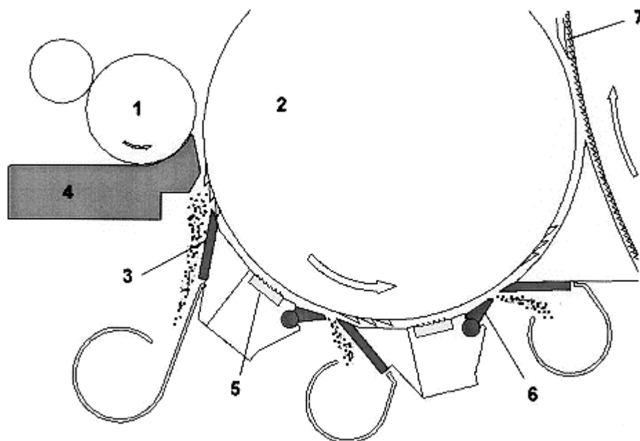
Fig. 22 Detail of the lick-in cylinder
