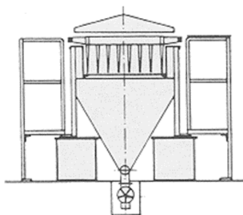
Fig. 119 – Scouring vats with two side settling troughs
