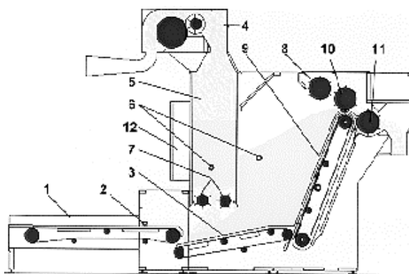
Fig. 6 Section of weighing feeder
