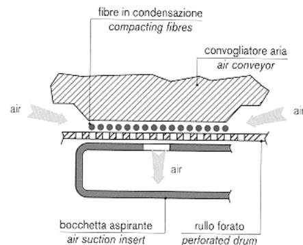
Fig. 234 - Air conveyor
