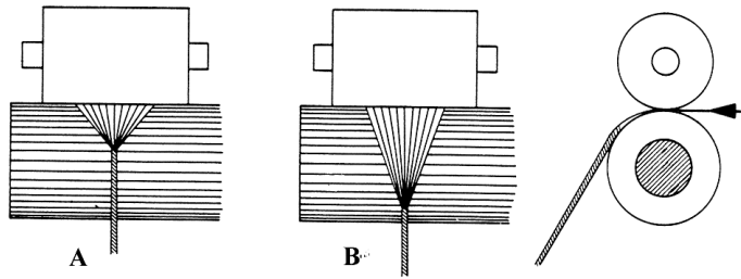
Fig. 228 - Spinning triangle
