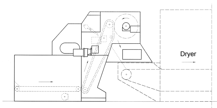
Fig. 127 – Automatic feeder connecting the two dryers
