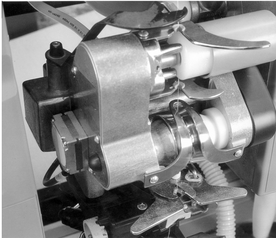
Fig. 60 Waxing device
