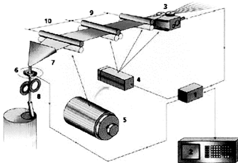
Fig. 30 Drawframe autoleveller
