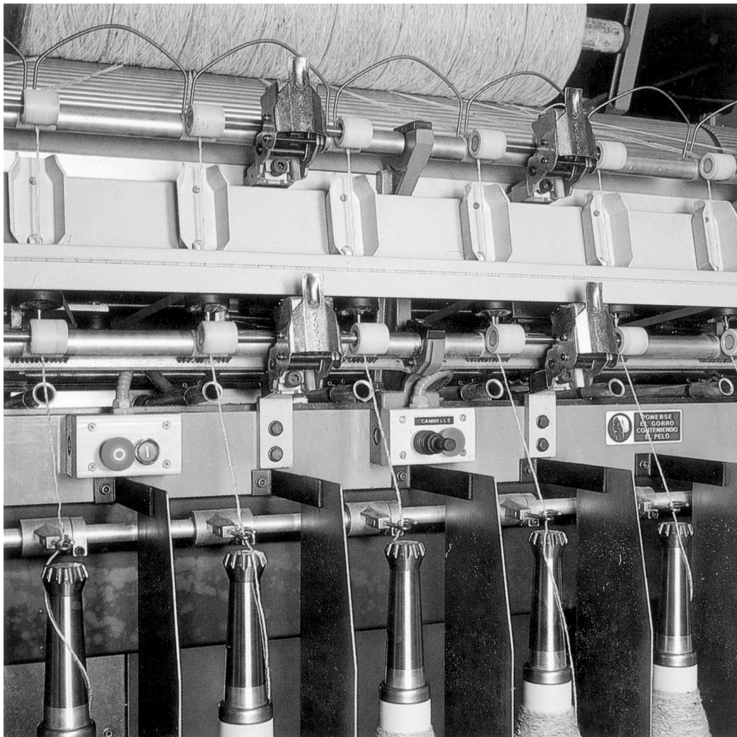
Fig. 89 Draft range and spinfinger
