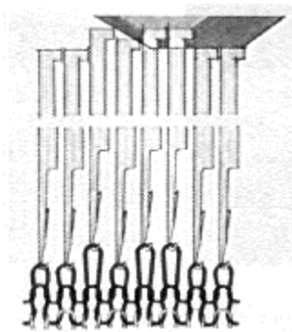
Picture 62 – Long and short stitches on the same course
