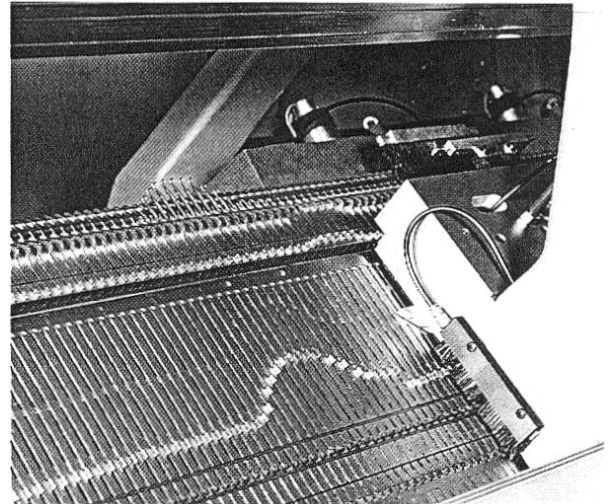
Picture 17 - The needle-bed of a flat knitting machine
