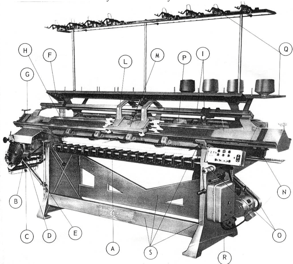
Picture 40 – Automatic flat knitting machine
