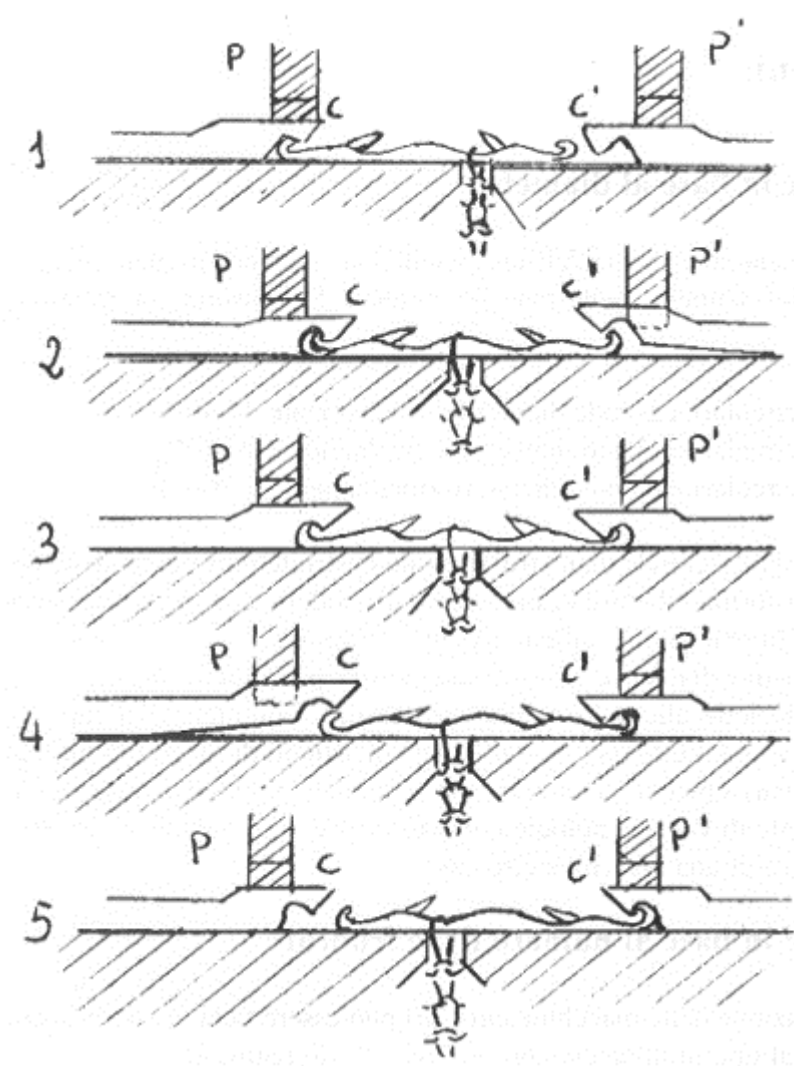
Picture 74 – The links-links knitting process
