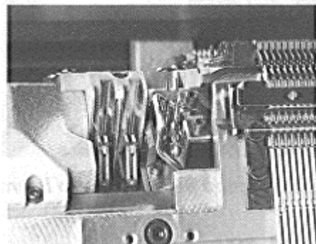
Picture 65 – Gripper and cutter unit
