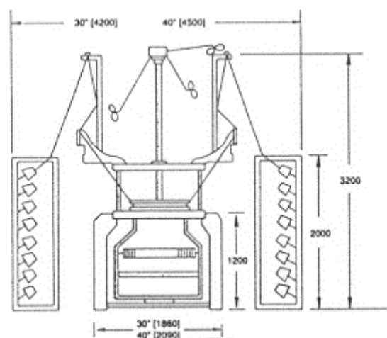
Picture 77 – Lateral creel
