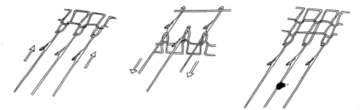
Picture 32 – Miss stitch formation
