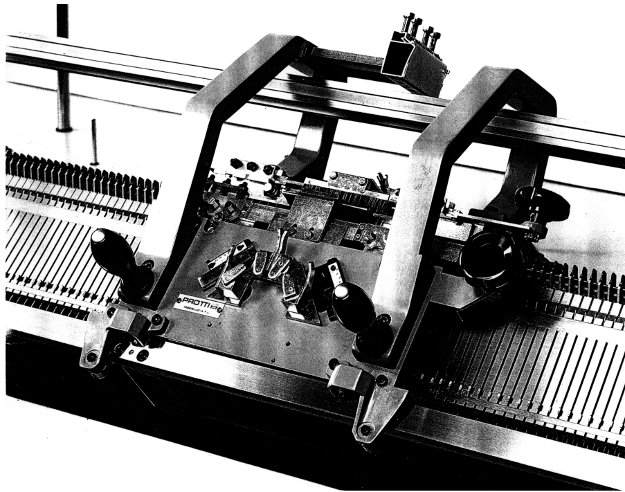
Picture 23 - Needle-bed and carriage of a manual flat knitting machine
