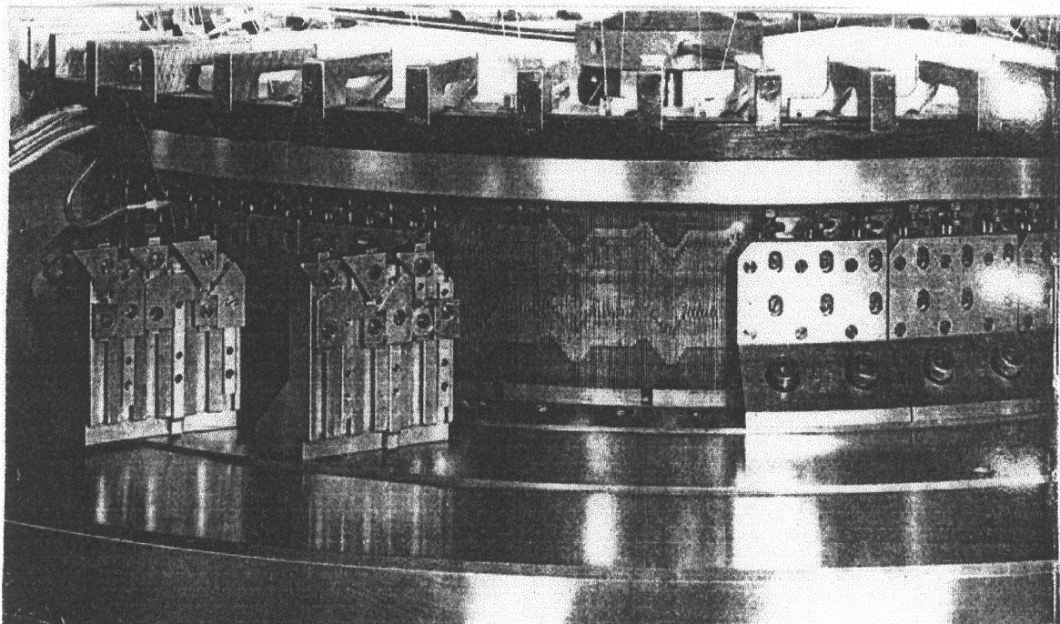
Picture 18 - The needle-bed of a circular knitting machine
