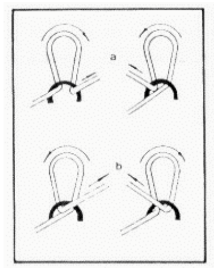
Picture 127 – Open (a) and closed (b) stitches
