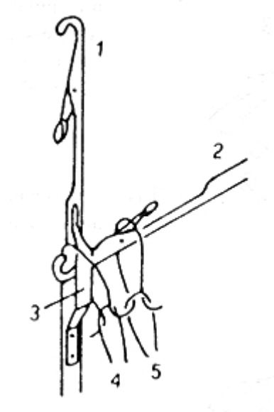
Picture 49 – Lateral spring transfer needle
