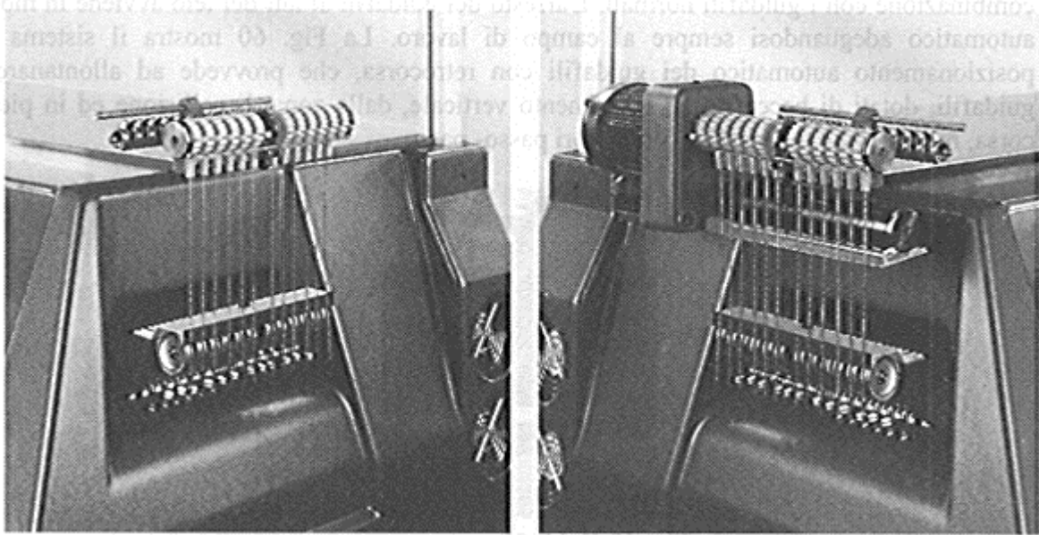
Picture 57/58 – Lateral tensioners
