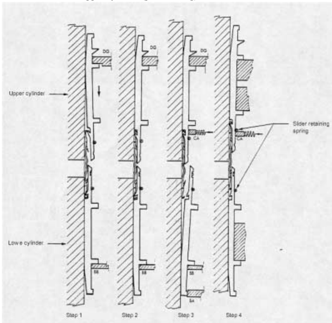
Picture 116 – Needle transfer on links machines
